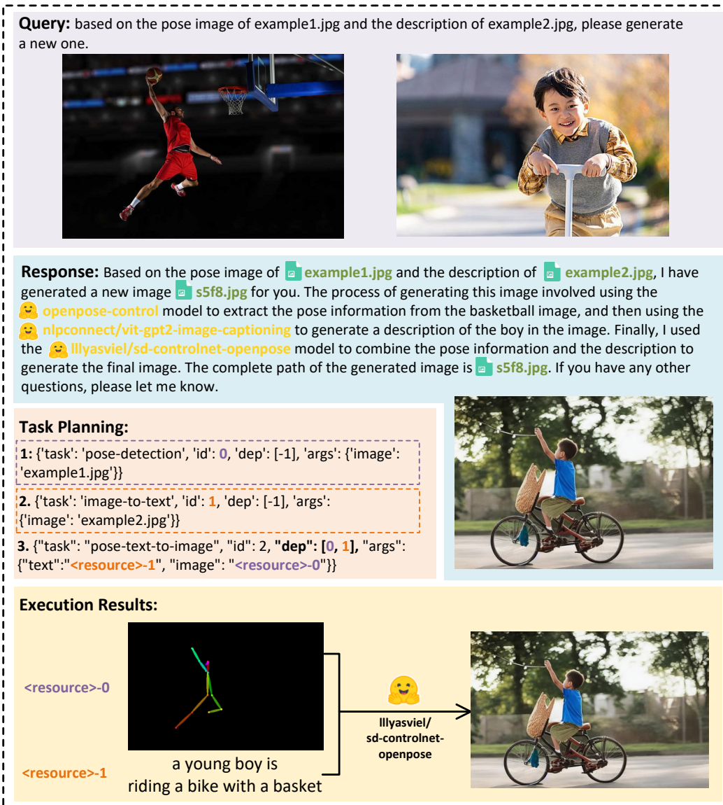
Figure 8: Qualitative analysis of multi-model cooperation with resource dependency.
